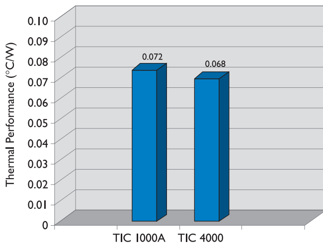
High Performance CPU Application, 38 × 38 mm
